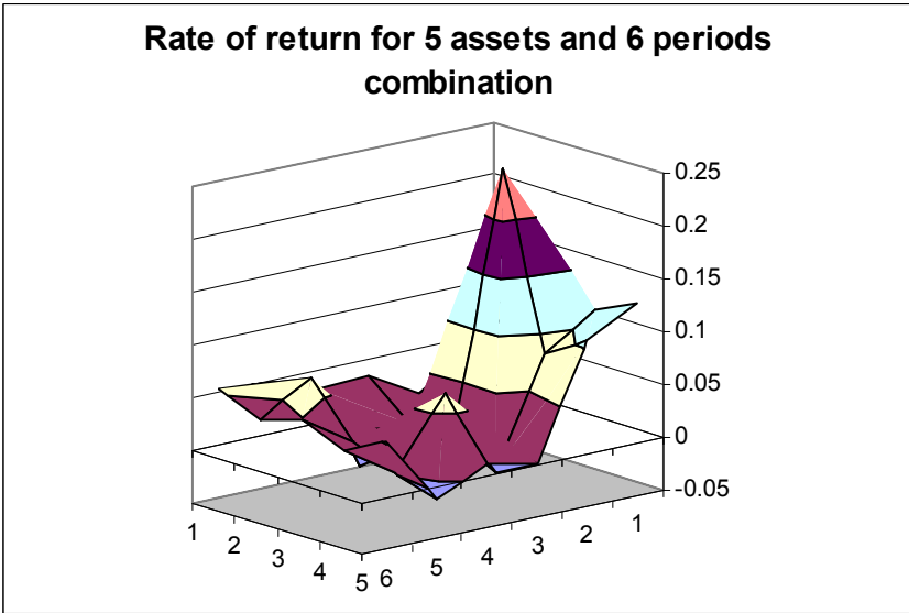
Fig. 8.5. Surface representing rates of return of period-asset combinations viewed from two perspectives.
