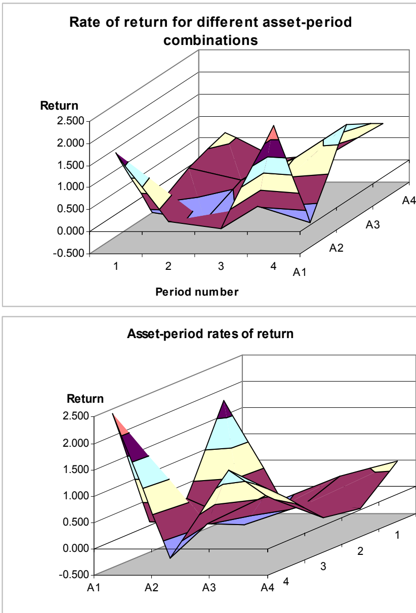
Fig. 8.3. Surface representing rates of return for period-asset combinations, viewed from different perspectives. A – assets' axis.
