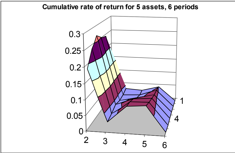
Fig. 8.6. Surface representing cumulative rates of return with accumulation across periods.
